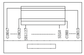
COM&SEG LAYOUT
