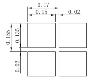
Detail A (20:1)
